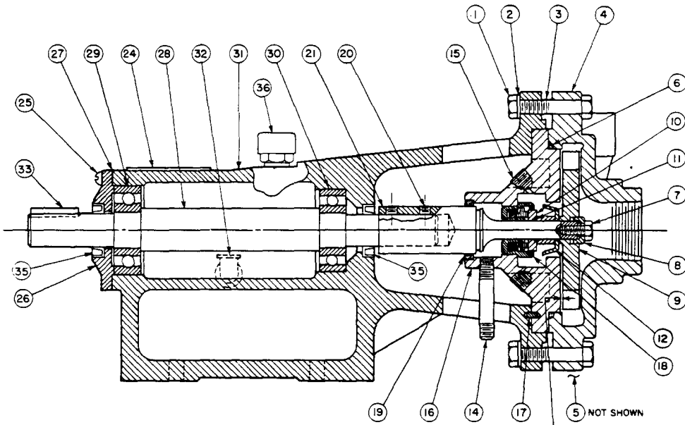
PEDESTAL MOUNTED
