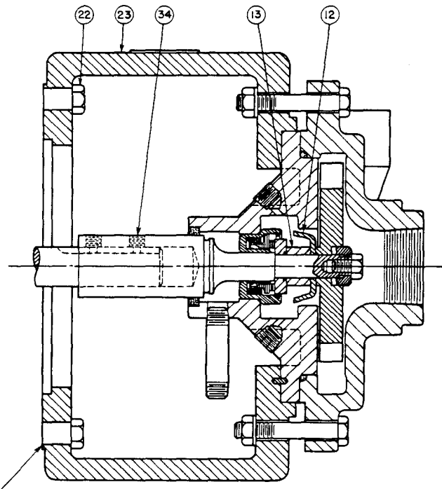
MOTOR MOUNTED
