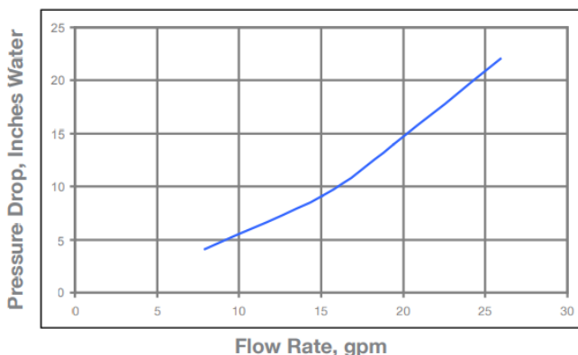
Pressure Drop of Improved Inline Mixers
